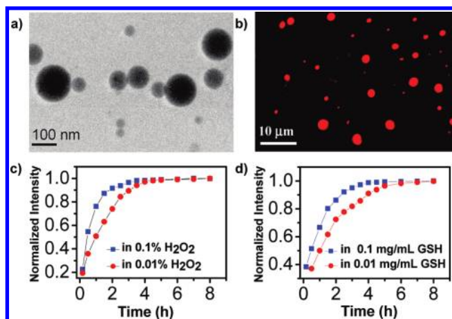
Figure 1. (a) Cryo-TEM image of PEG-PUSeSe-PEG micelles. (b) FM image of RB-loaded micelles, and the release behavior of RB in (c) H 2 O 2 and (d) GSH.
